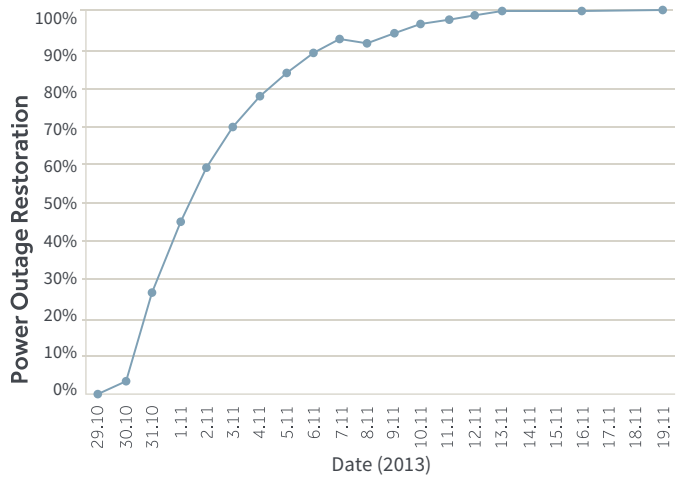
Figure 2. Restoration of power outage for affected customers in the US Source: Kunz et al. (2013). Data from U.S. Department of Energy, Office of Electricity Delivery and Energy Reliability
